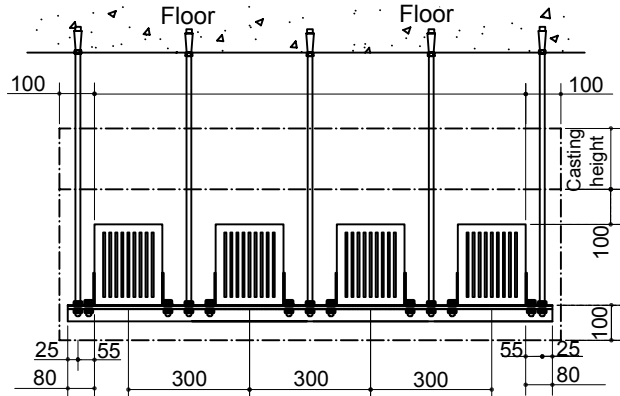
Cross-sectional Diagram of Quadruple-Busbar (Unit: mm)
