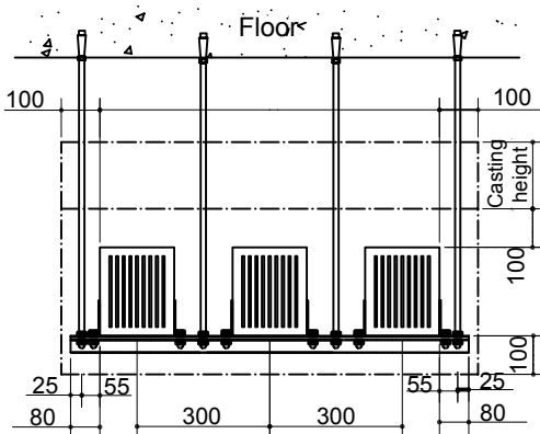
Cross-sectional Diagram of Triple-Busbar (Unit: mm)
