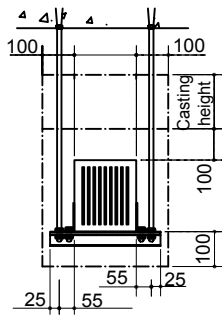
Cross-sectional Diagram of Single-Busbar (Unit: mm)
