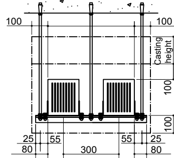
Cross-sectional Diagram of Dual-Busbar (Unit: mm)
